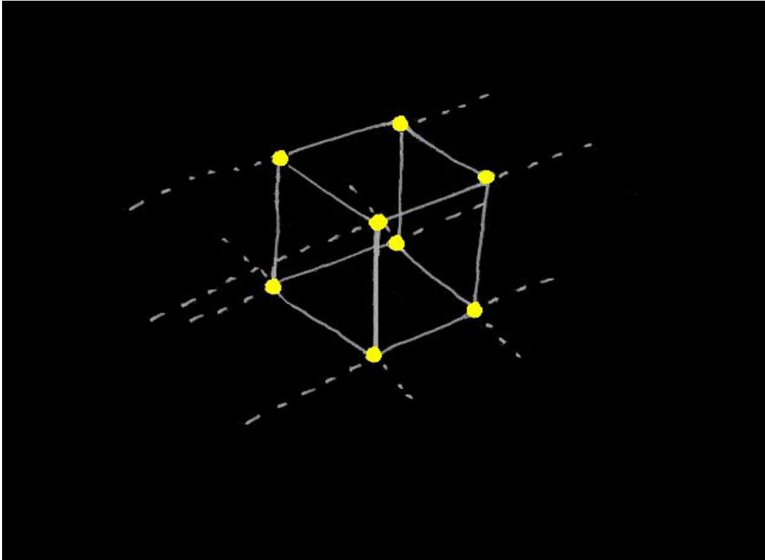
Plate 1.2: Single Lattice cube of bound Quantum Particles (the yellow dots) that make up the Material Cause
