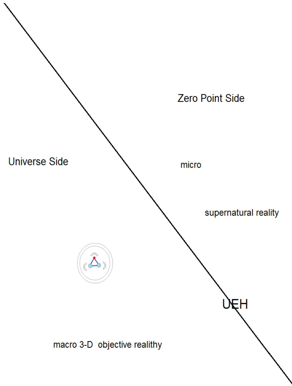
Diagram 1.2: The Universe Event Horizon (UEH) or the boundary between the objective, measurable reality we live in and the subjective, supernatural reality of the Quantum Field
